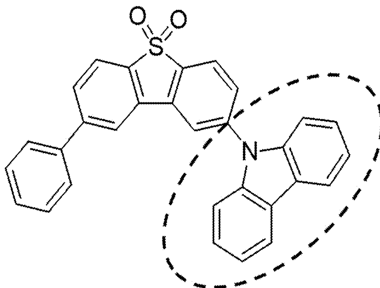
Carbazole
