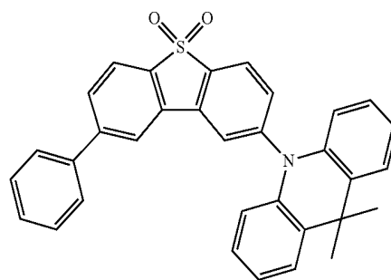
[Formula 7]
