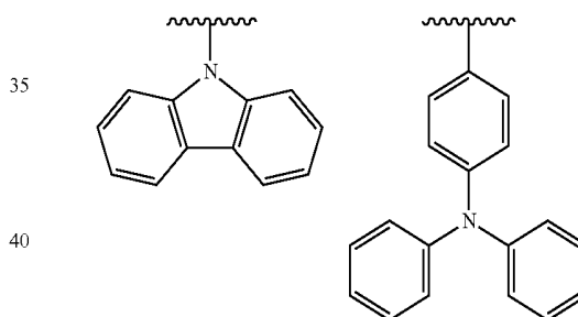
[Formula 6]
