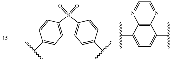
[Formula 2]
