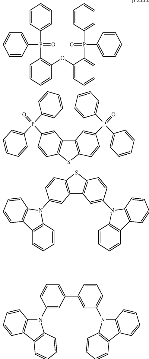
[Formula 9]
