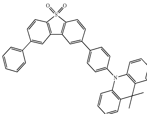
compound 3
